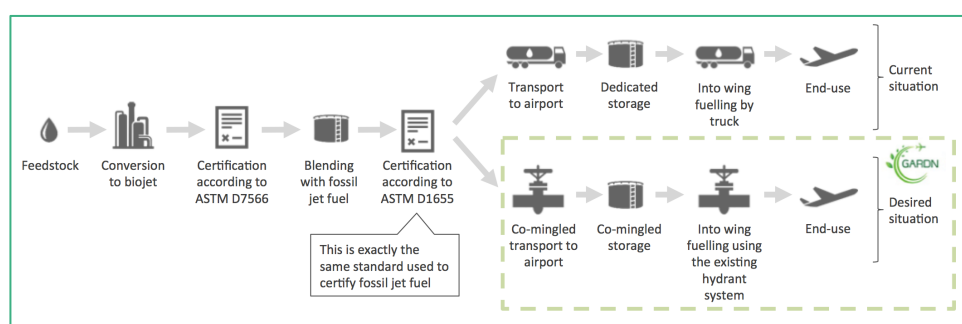
FIGURE 5-3 CBSCI Project Overview (Source: SkyNRG, 2017)
