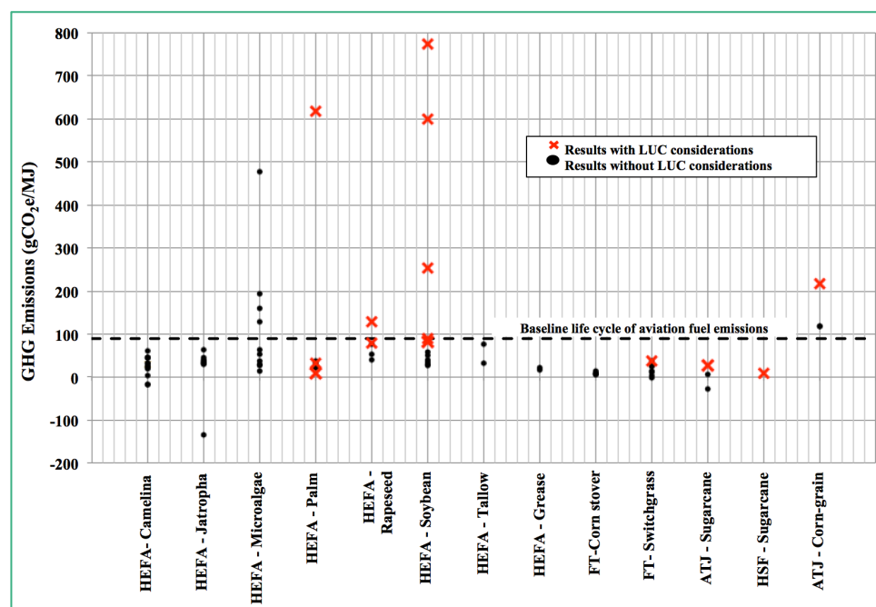
FIGURE 4-4 Main results from LCA studies for aviation fuels. (Source: Adapted from Capaz and Seabra, 2016)
