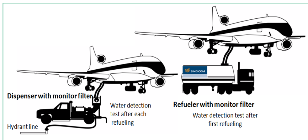
FIGURE 5-6 Quality control procedures at airport apron (Source: Schumman, 2013)
