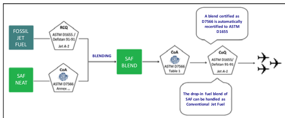
FIGURE 9 Blending and use process for SAFs synthetic fuels and quality standards 60
