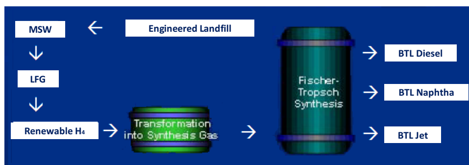
FIGURE 11 Key technology components for BTL-FT synthesis
