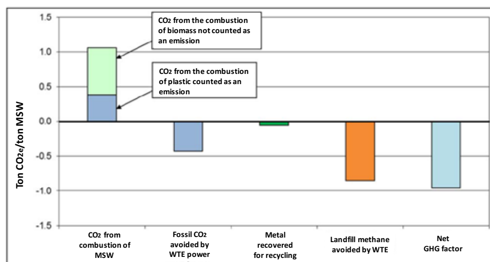
FIGURE 12 Waste to energy LCA testing results 108
