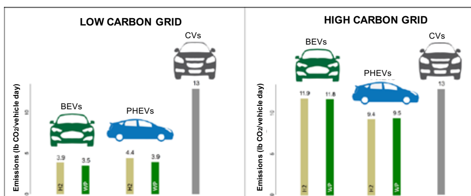
FIGURE 6 Comparison of total BEV200 and PHEV CO 2 emissions with emissions from a CV on a low and high carbon grid 34 .
